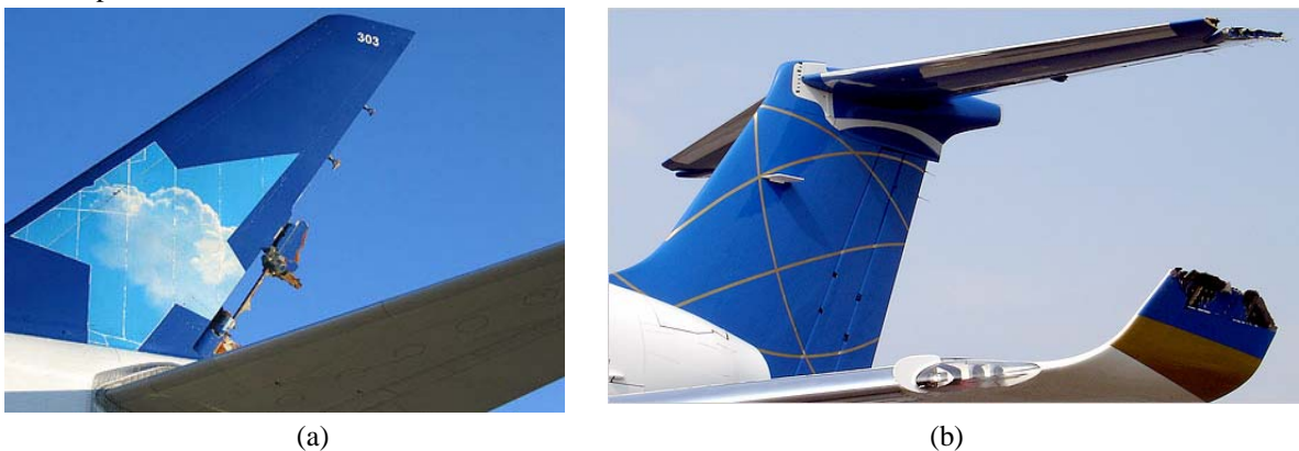
Figure 1 (a) Air Transat A310 - 2005 - Rudder Loss; (b) Embraer Legacy 600 – Brazil – Wing Tip and Stabilator Loss, September 2006.
